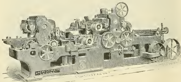
No. 106. DOUBLE CYLINDER "LIGHTNING" FLOORER.
